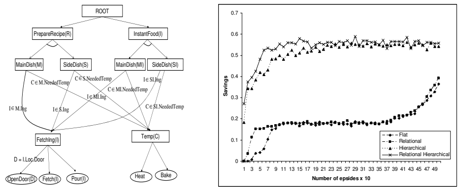
Fig. 4. (a)The kitchen domain hierarchy. (b)Learning curves of the different algorithms in the Kitchen Domain.
