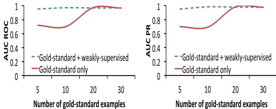
Fig. 5. Results of classifying football and soccer articles in the Document Classification domain: (Left) AUC ROC. (Right) AUC PR.
